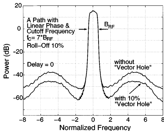
Fig. 11. Spectra of the digital signal: cutoff frequency of a path seven times the RF bandwidth.
