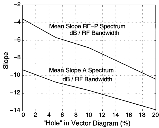
Fig. 8. Slopes of A and RF-P signals as a function of the radius of the hole in the vector diagram.
