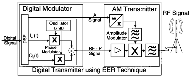
Fig. 1. Structure of an EER transmitter.
