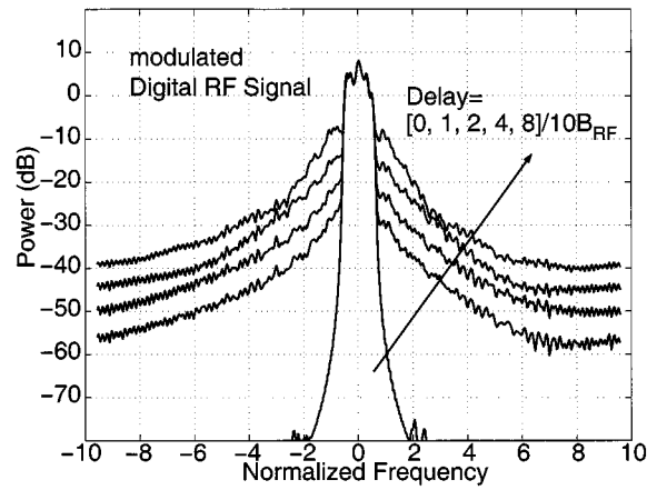
Fig. 9. Spectra of the modulated digital RF signal for various delays (without a vector hole).
