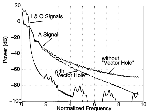
Fig. 4. Spectra of the I &amp; Q and A signals.
